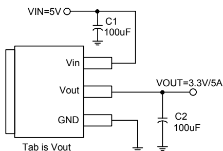
5.0V to 3.3V Fixed Mode Regulator
