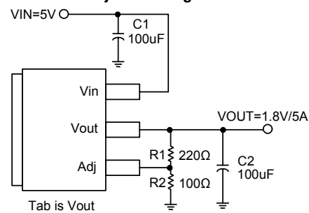
Adjustable Regulator
