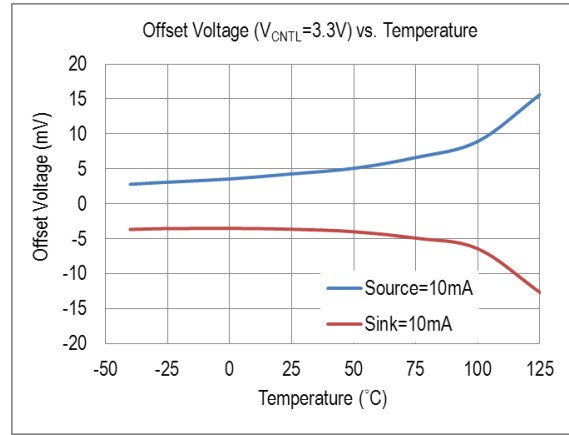
DDR-III
