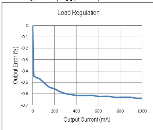
Load Regulation V IN =3.6V, V OUT =1.2V, L=2.2μH
