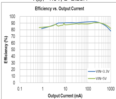
Efficiency vs. Output Current V OUT =1.8V, L=2.2μH
