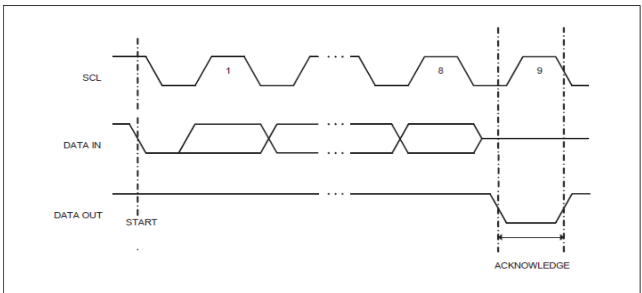
Figure 3: Output Acknowledge
