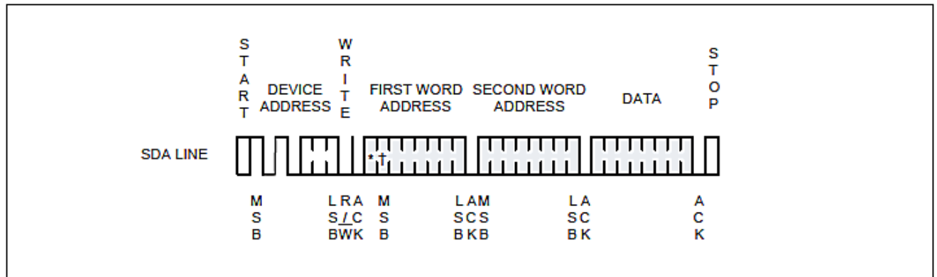
Figure 6: Page Write
