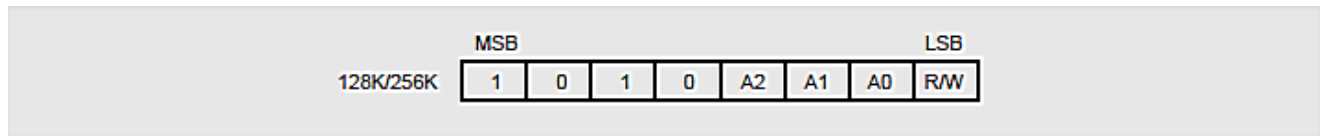
Figure 5: Byte Write
