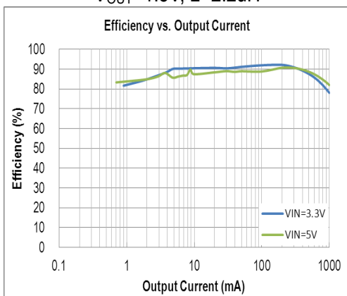
Efficiency vs. Output Current V_{OUT}=1.8V, L=2.2uH
