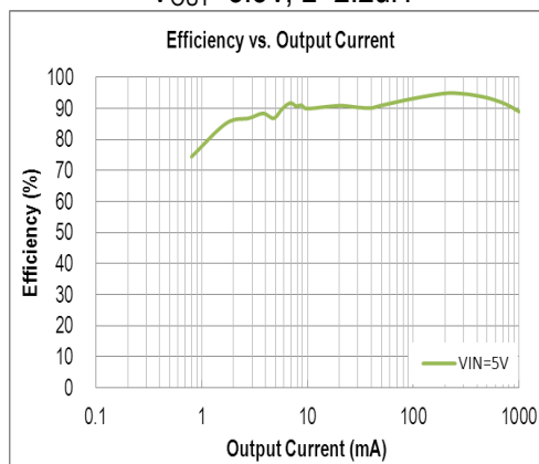
Efficiency vs. Output Current V_{OUT}=3.3V, L=2.2uH
