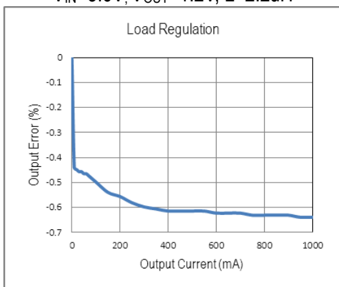
Load Regulation V_{IN}=3.6V, V_{OUT}=1.2V, L=2.2uH
