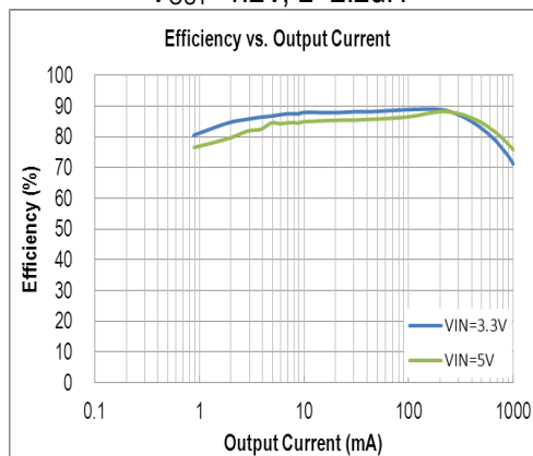
Efficiency vs. Output Current V_{OUT}=1.2V, L=2.2uH
