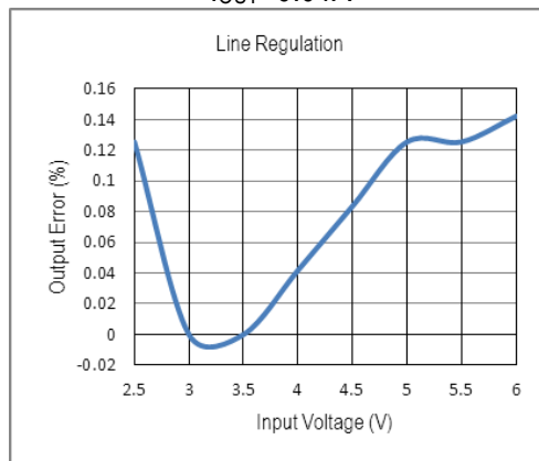
Line Regulation I_{OUT}=0.01A
