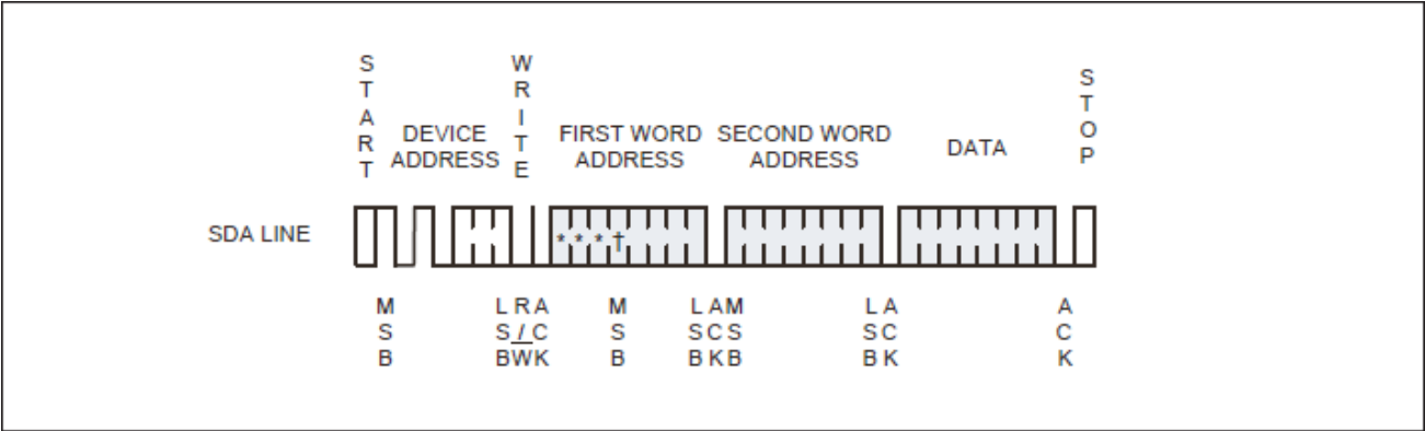
Figure 5: Byte Write
