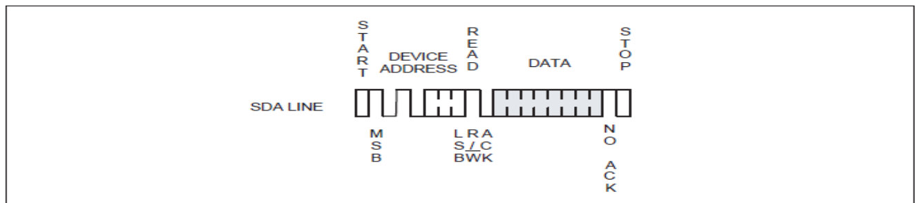
Figure 8: Random Read
