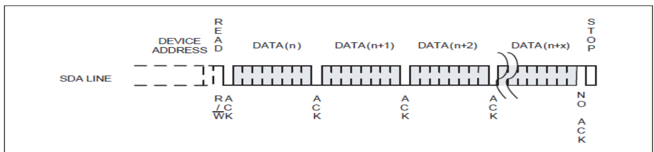
Figure 9: Sequential Read
