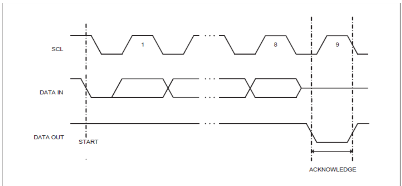
Figure 3: Output Acknowledge
