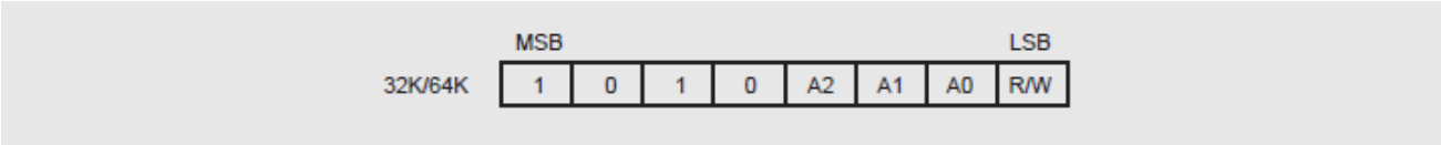
Figure 5: Byte Write
