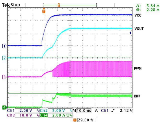
Power-ON Wave (VCC=5V, VOUT=12V, Load=0.7A, SS=0.1uF)
