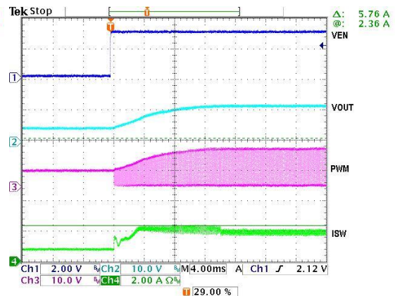
Enable-ON Wave (VCC=5V, VOUT=12V, Load=0.7A, SS=0.1uF)
