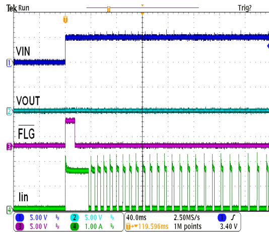
output short circuit &amp; over temperature protection
