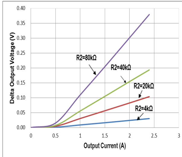
Figure2 12Vin to 5Vout Cable Compensation (RSEN=33mΩ)
