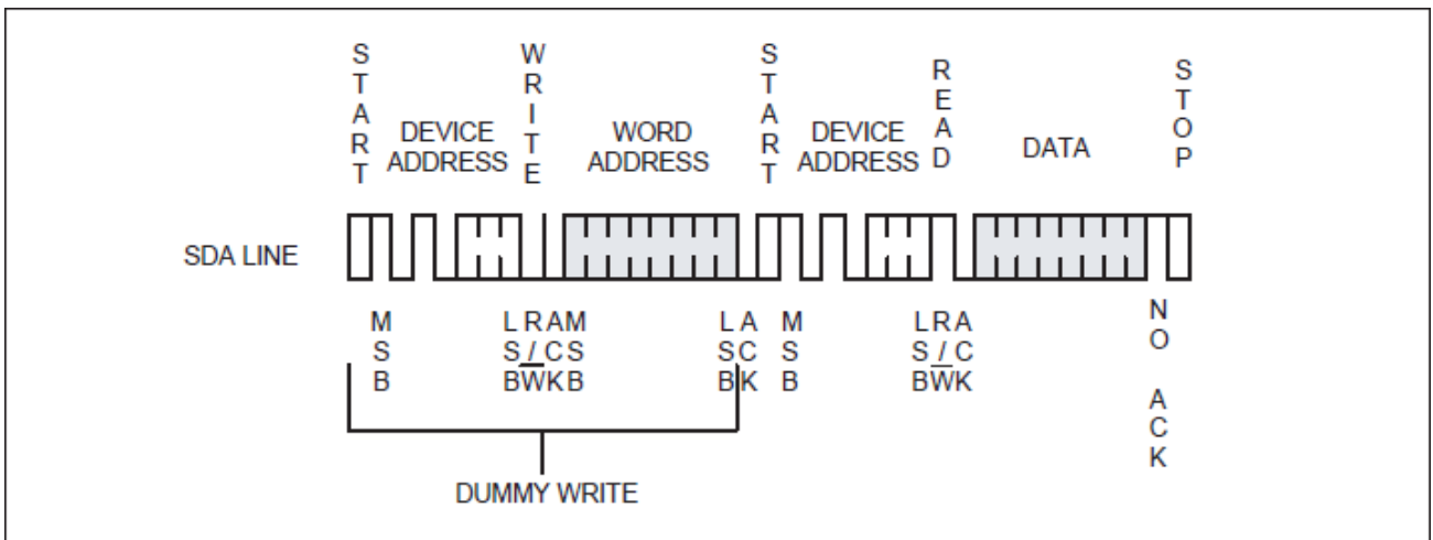
Figure 8: Random Read
