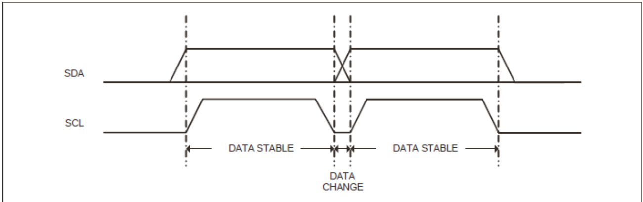
Figure 1: Data Validity
