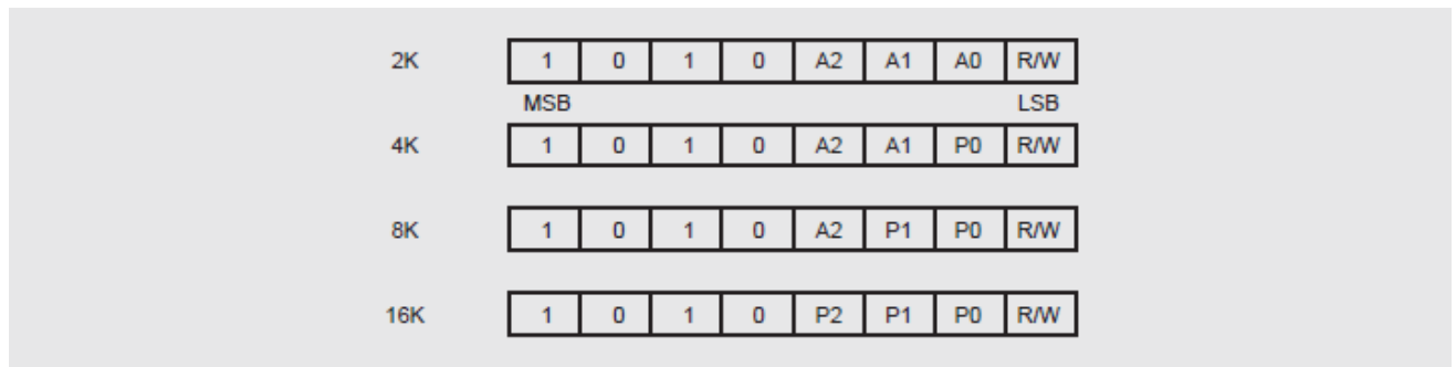
Figure 4: Device Address
