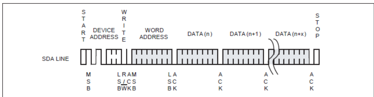
Figure 6: Page Write
