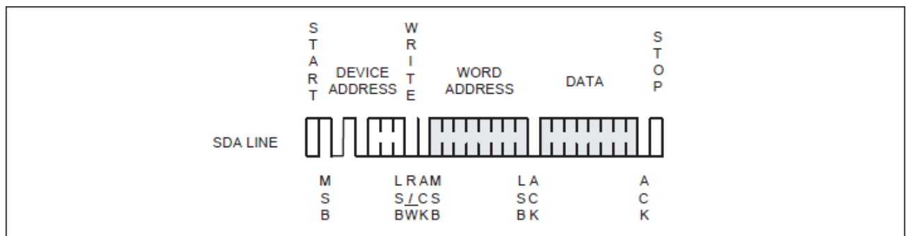
Figure 5: Byte Write
