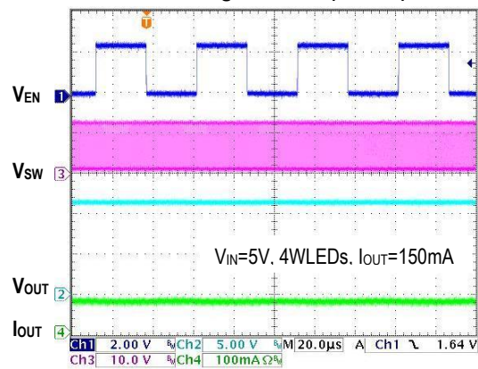
PWM Dimming from EN (20KHz)
